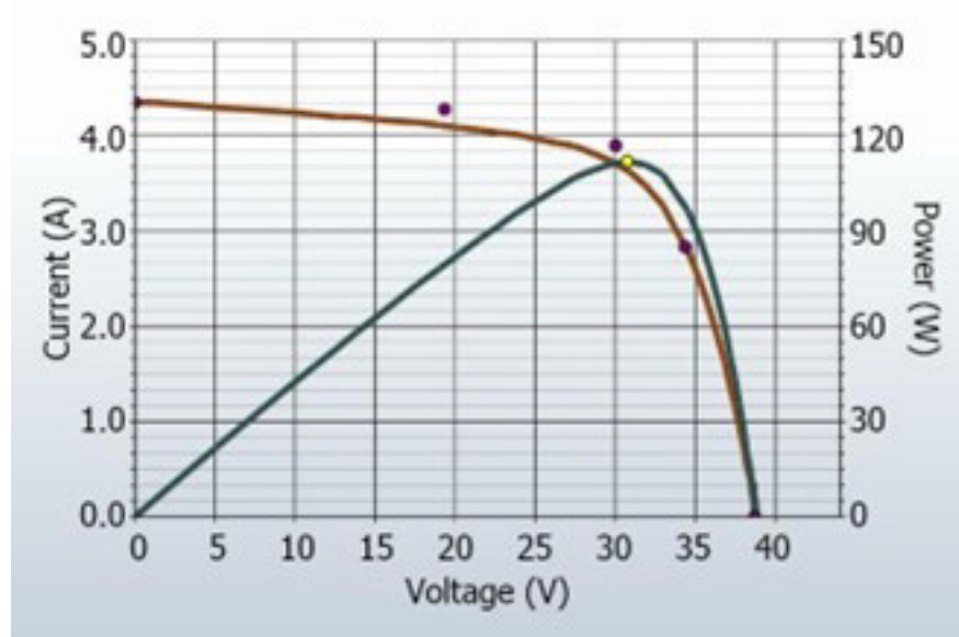
Figure 20. I-V Curve with a Steeper Slope in the Horizontal Leg of the I-V Curve
